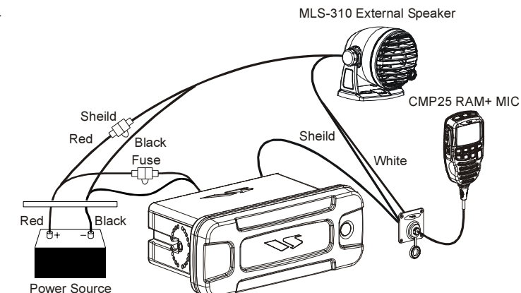
Phantom Series Connections
